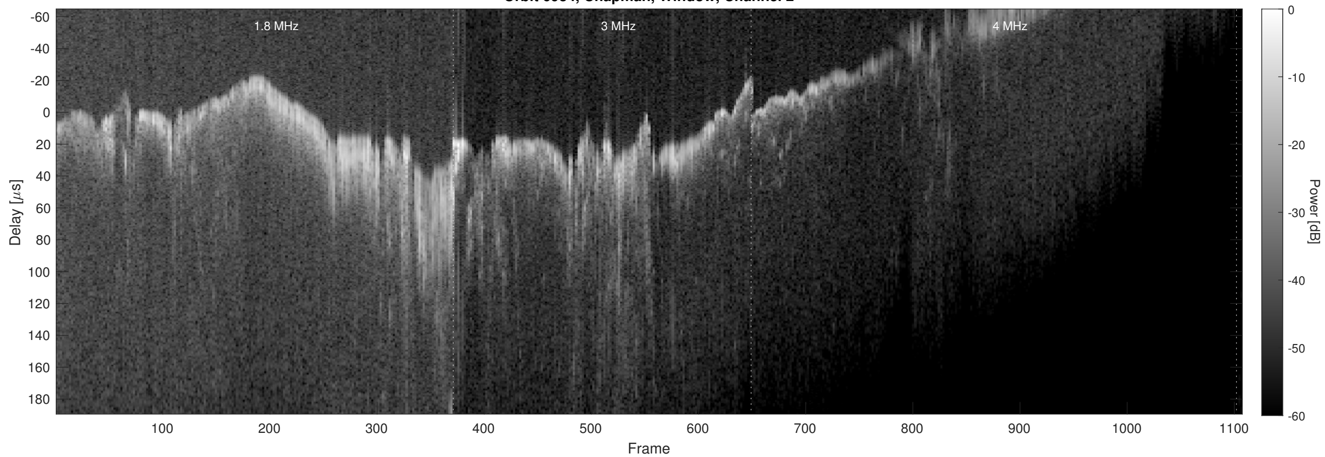
Orbit 6934, Chapman, Window, Channel 2
