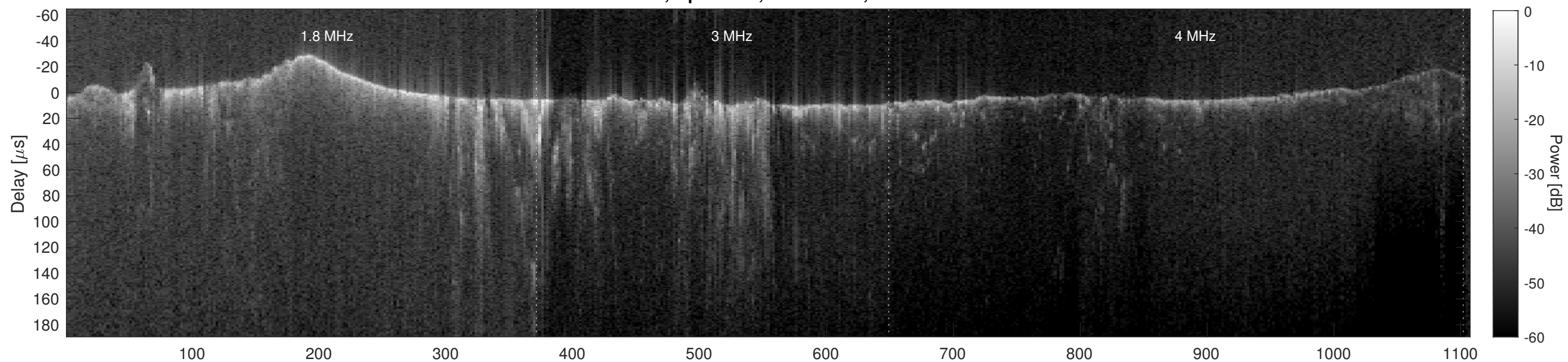
Orbit 6934, Cluttergram
