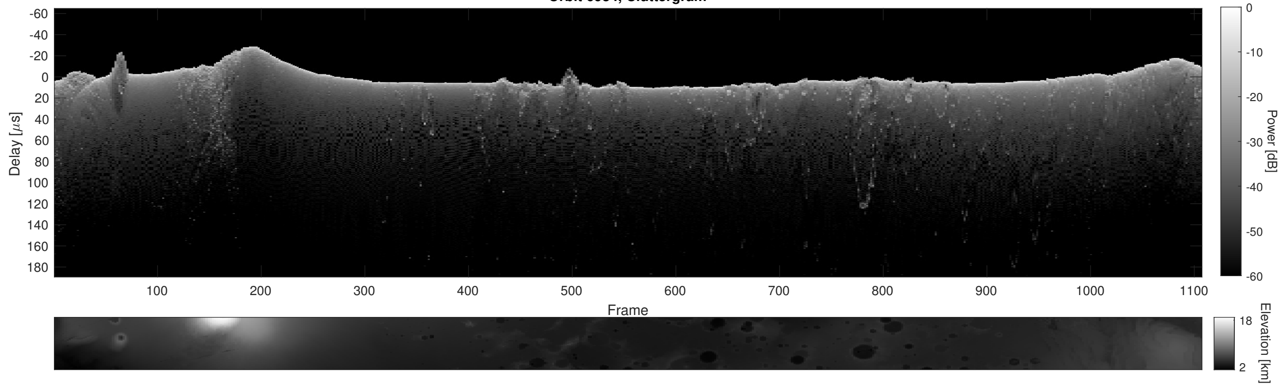
Orbit 6934, Cluttergram
