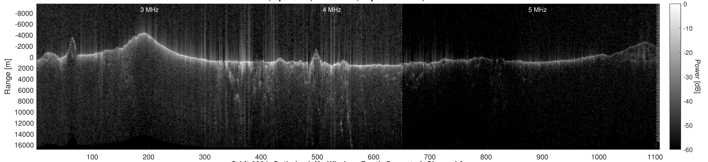
Orbit 6934, Optimized, No Window, Depth-Corrected, Channel 2
