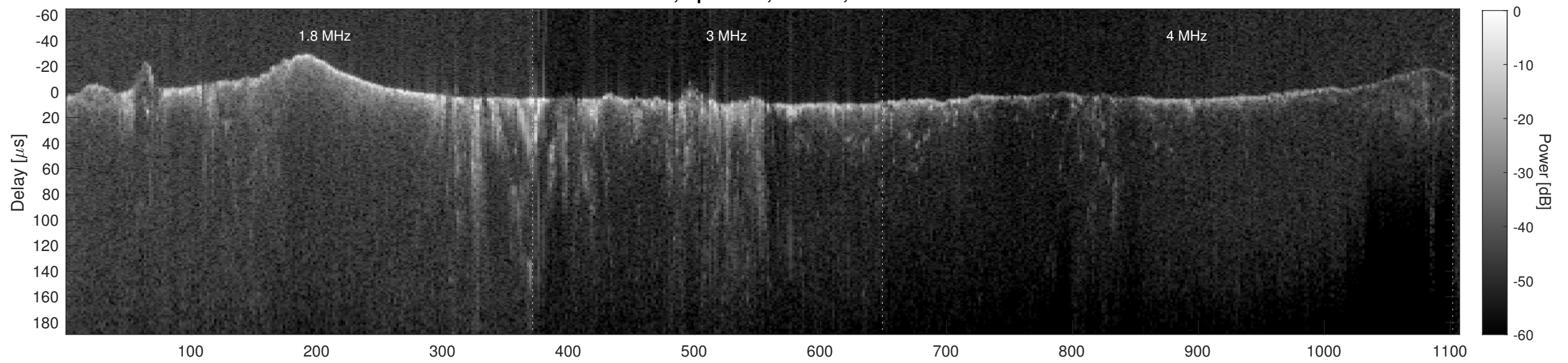
Orbit 6934, Cluttergram
