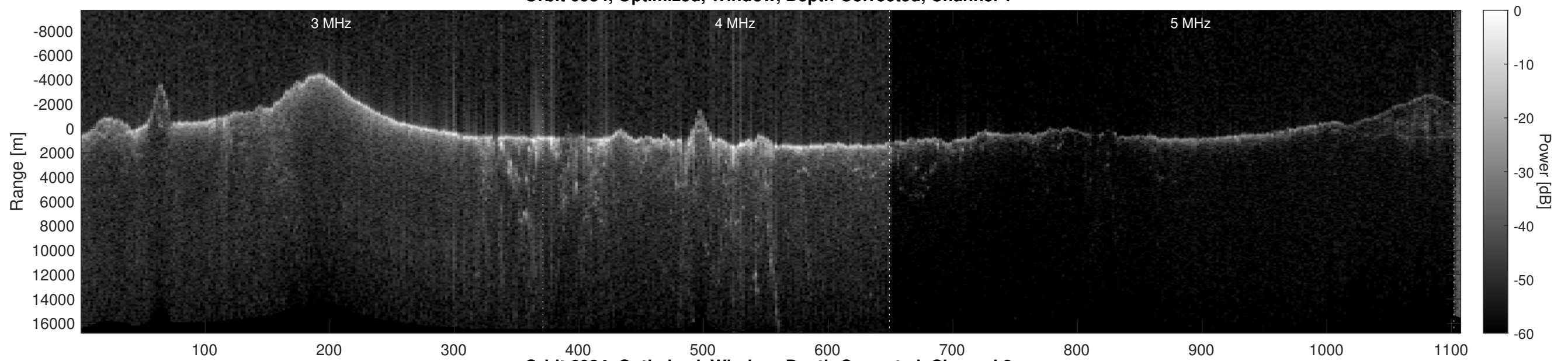
Orbit 6934, Optimized, Window, Depth-Corrected, Channel 2
