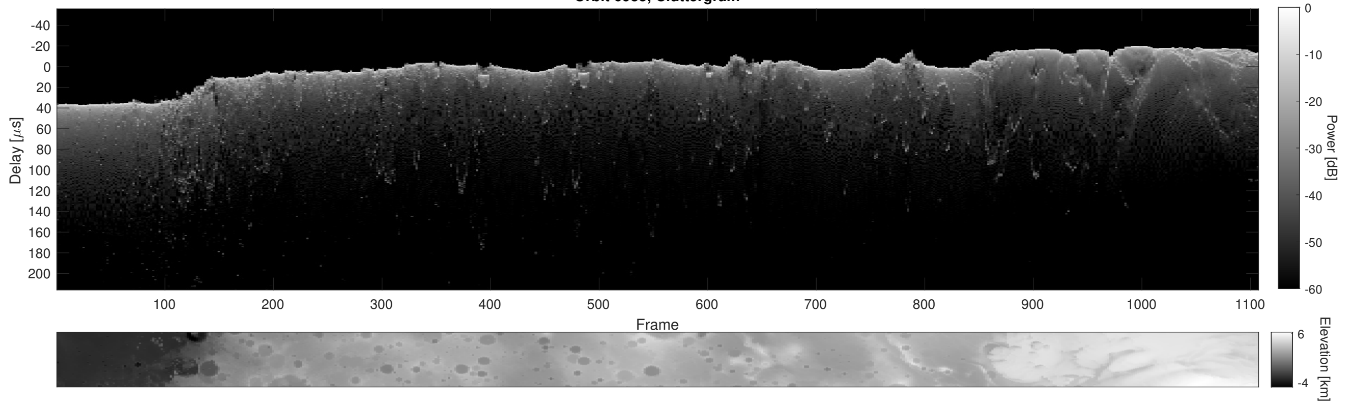
Orbit 6935, Cluttergram
