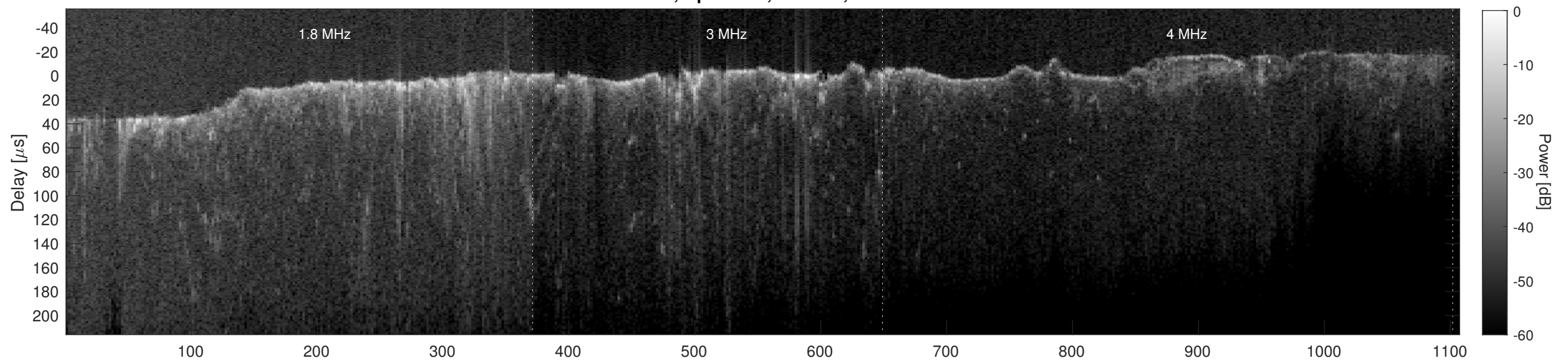
Orbit 6935, Cluttergram
