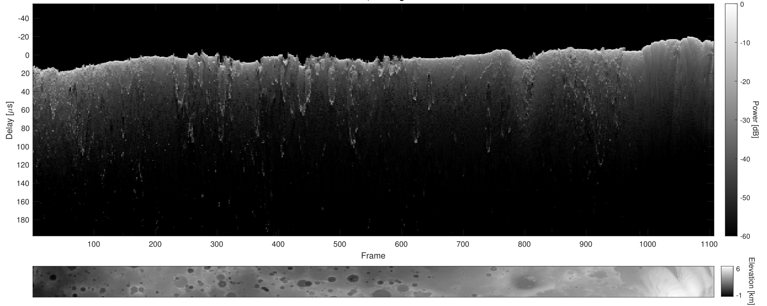
Orbit 6936, Cluttergram
