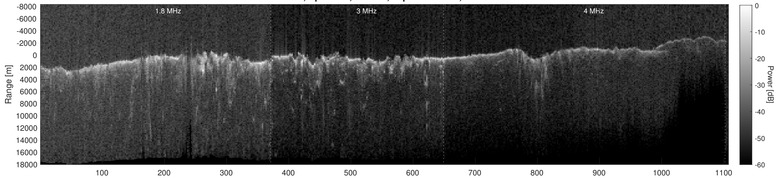
Orbit 6936, Depth-Corrected Cluttergram
