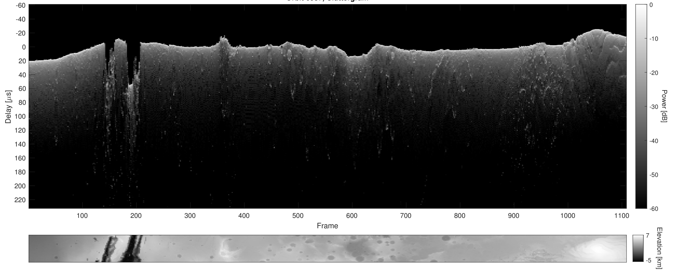
Orbit 6937, Cluttergram
