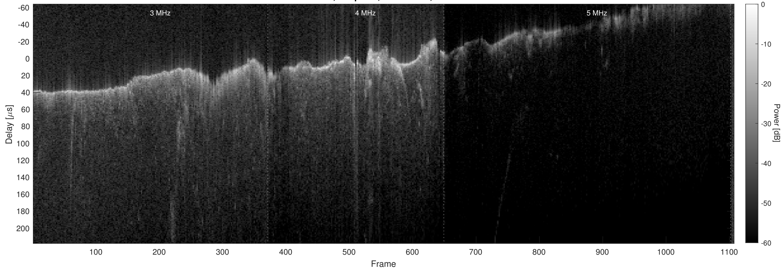
Orbit 6938, Chapman, No Window, Channel 2
