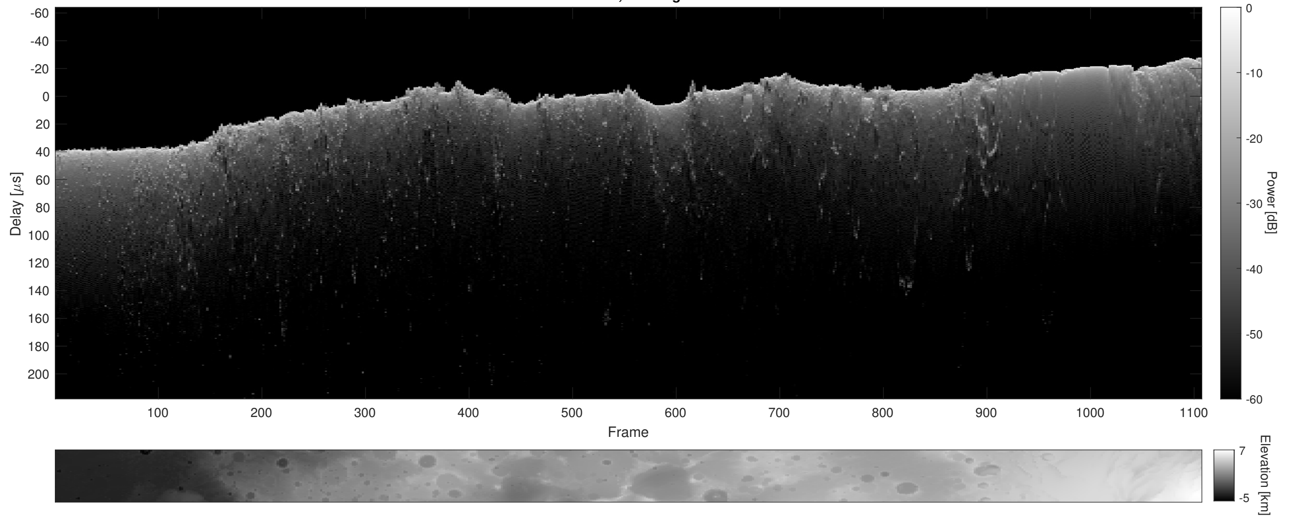
Orbit 6938, Cluttergram
