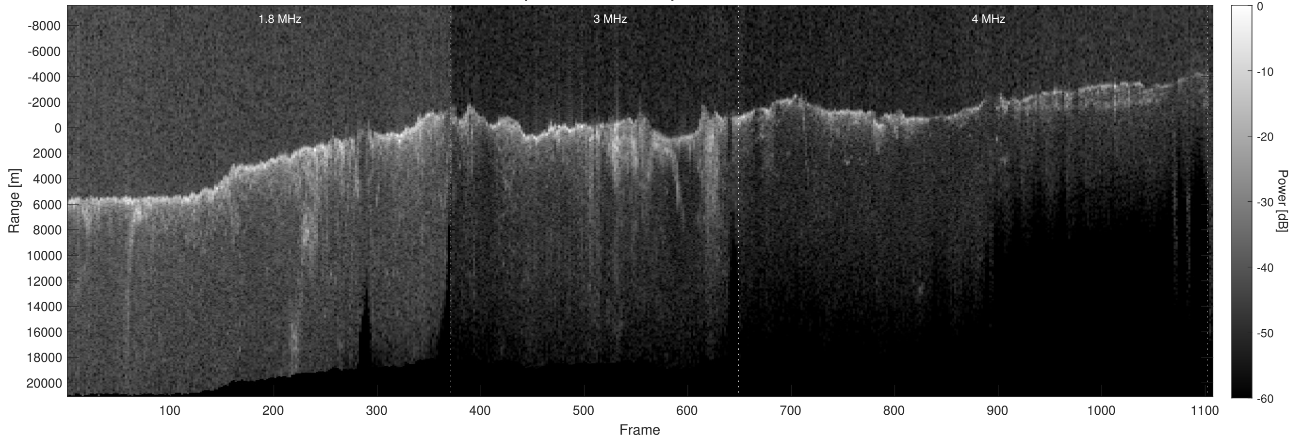
Orbit 6938, Optimized, Window, Depth-Corrected, Channel 2
