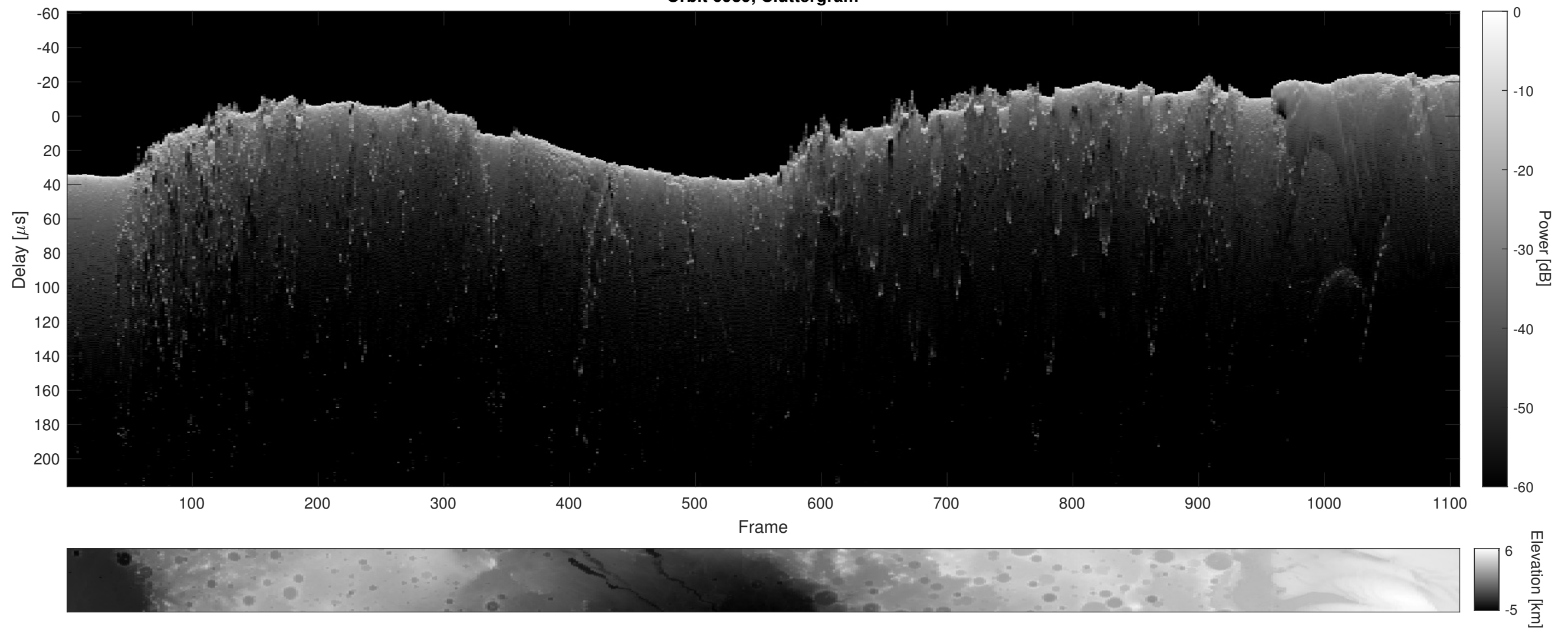
Orbit 6939, Cluttergram
