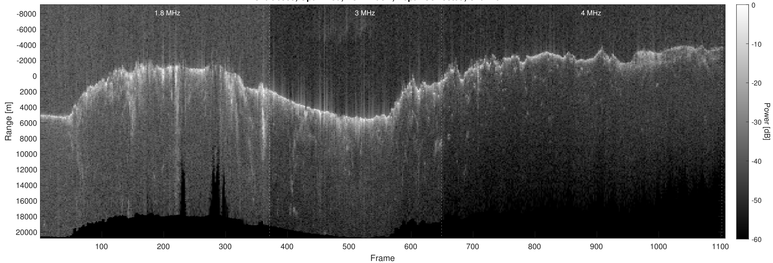
Orbit 6939, Optimized, No Window, Depth-Corrected, Channel 2
