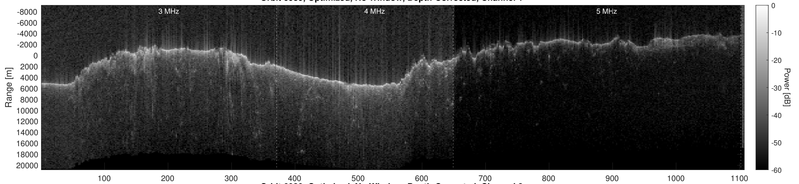
Orbit 6939, Optimized, No Window, Depth-Corrected, Channel 2
