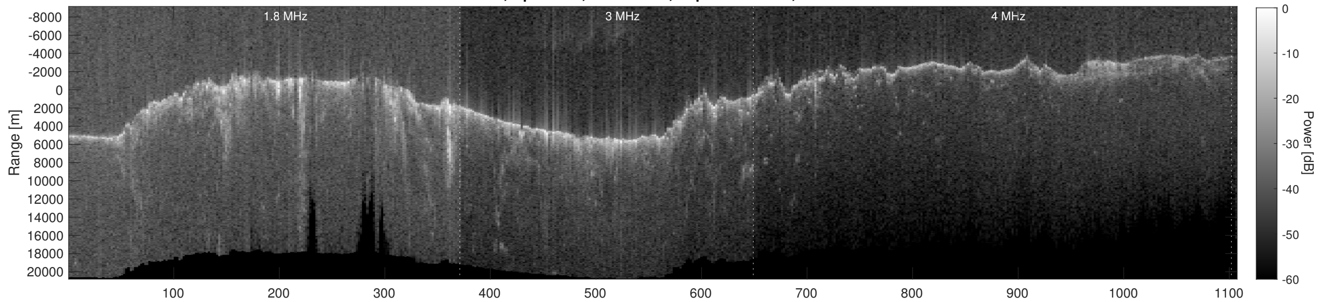
Orbit 6939, Depth-Corrected Cluttergram
