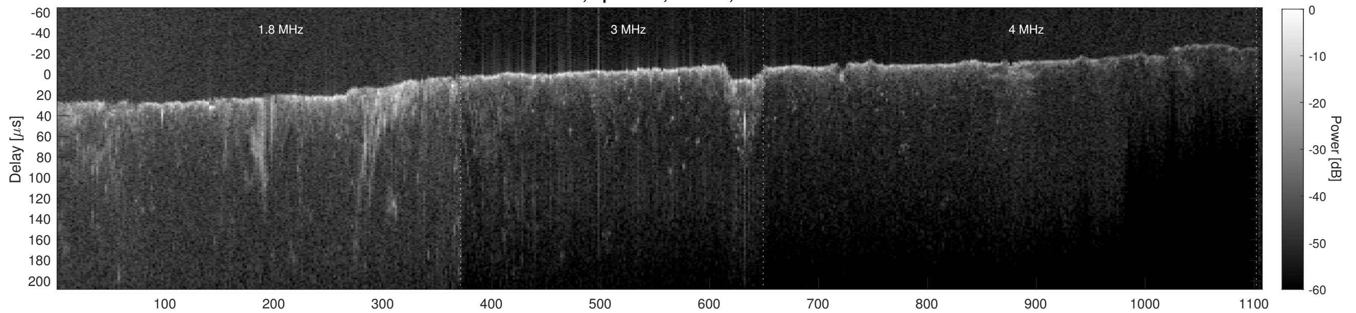
Orbit 6940, Cluttergram
