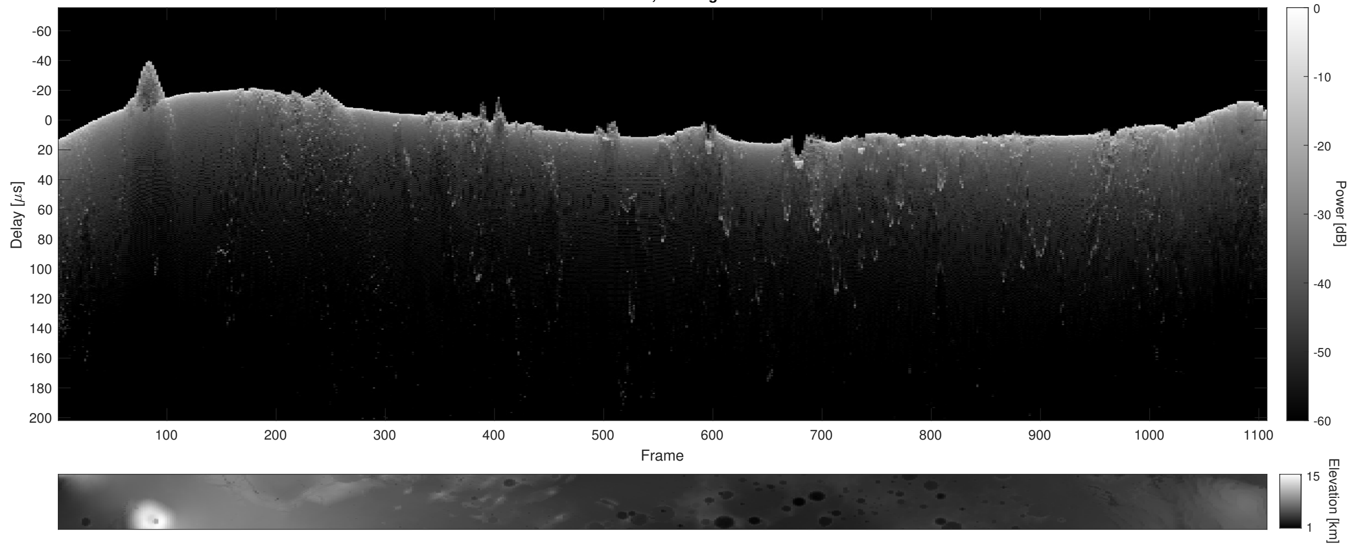
Orbit 6941, Cluttergram
