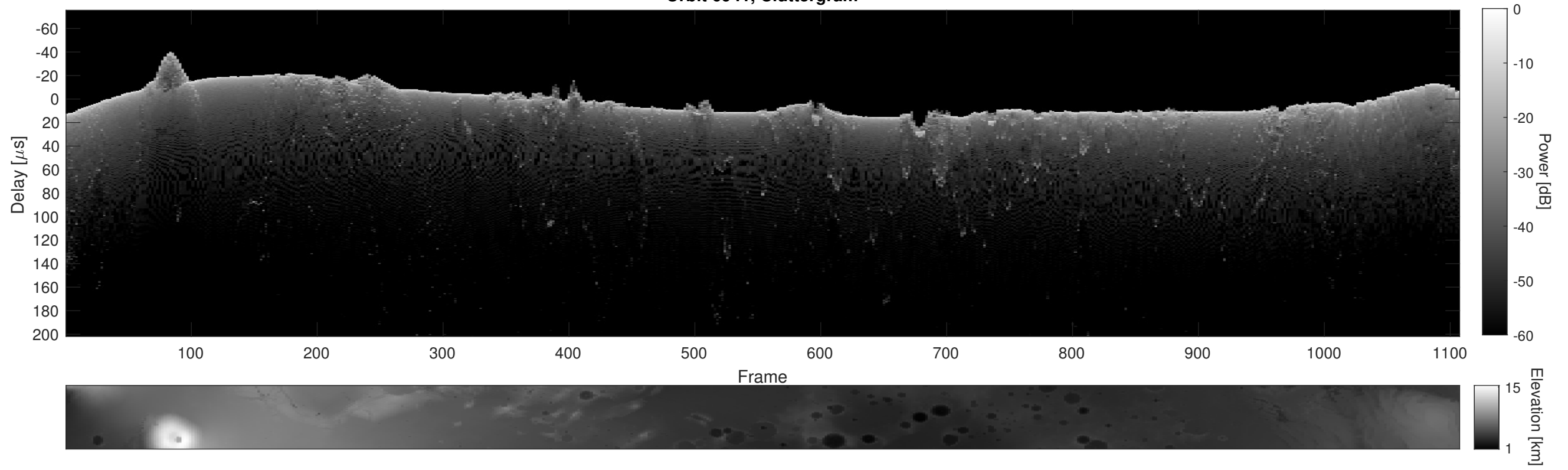
Orbit 6941, Cluttergram
