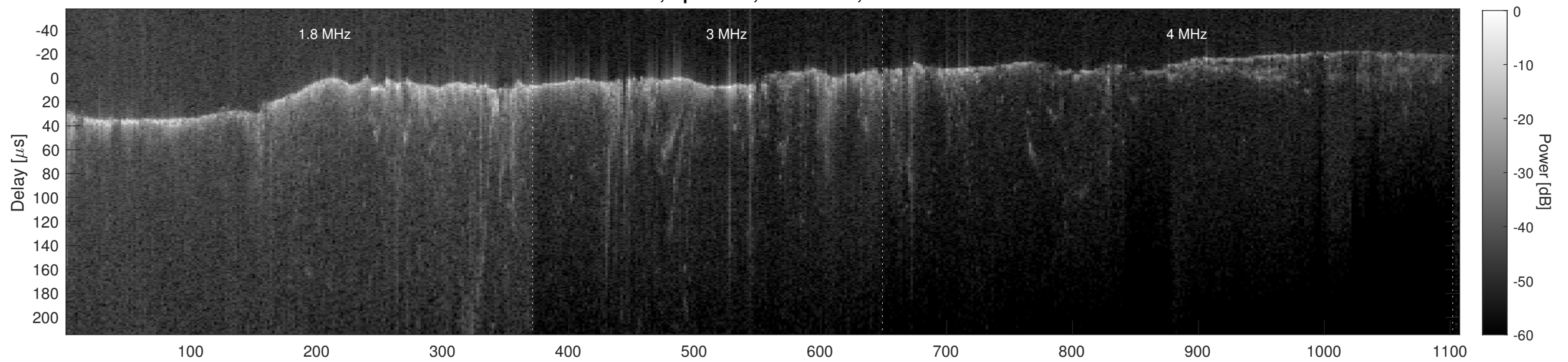
Orbit 6942, Cluttergram
