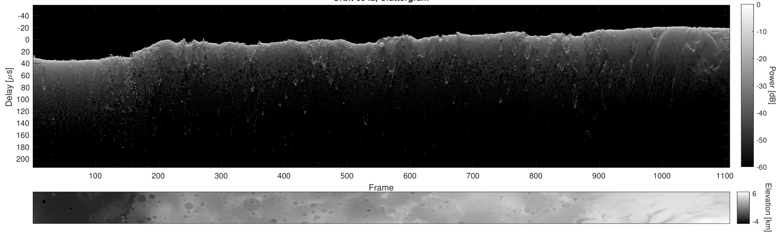
Orbit 6942, Cluttergram
