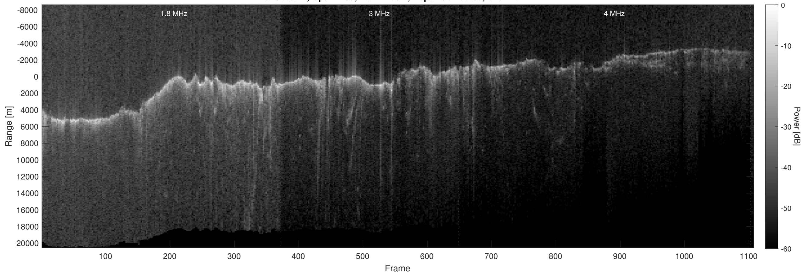
Orbit 6942, Optimized, No Window, Depth-Corrected, Channel 2
