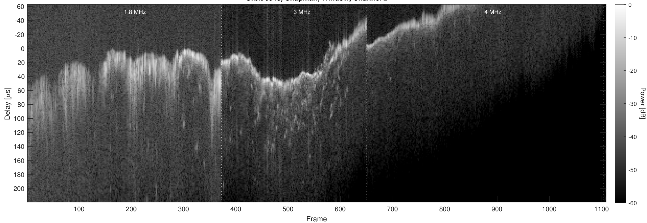
Orbit 6943, Chapman, Window, Channel 2
