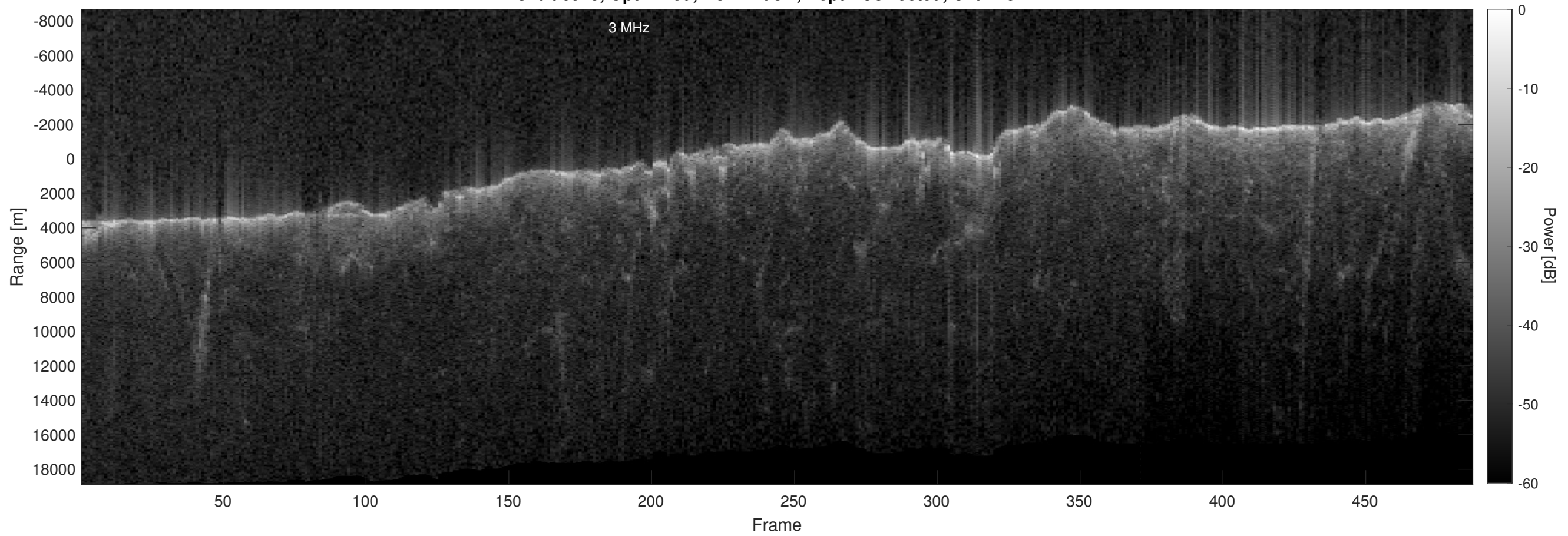
Orbit 6945, Optimized, No Window, Depth-Corrected, Channel 2
