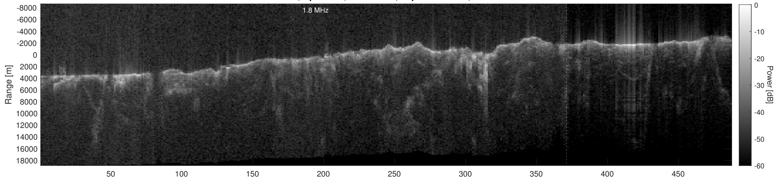
Orbit 6945, Depth-Corrected Cluttergram
