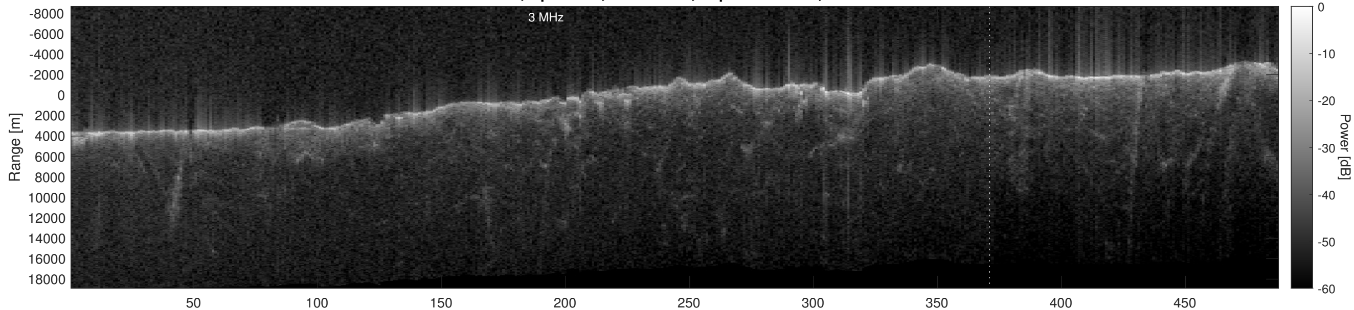
Orbit 6945, Optimized, No Window, Depth-Corrected, Channel 2
