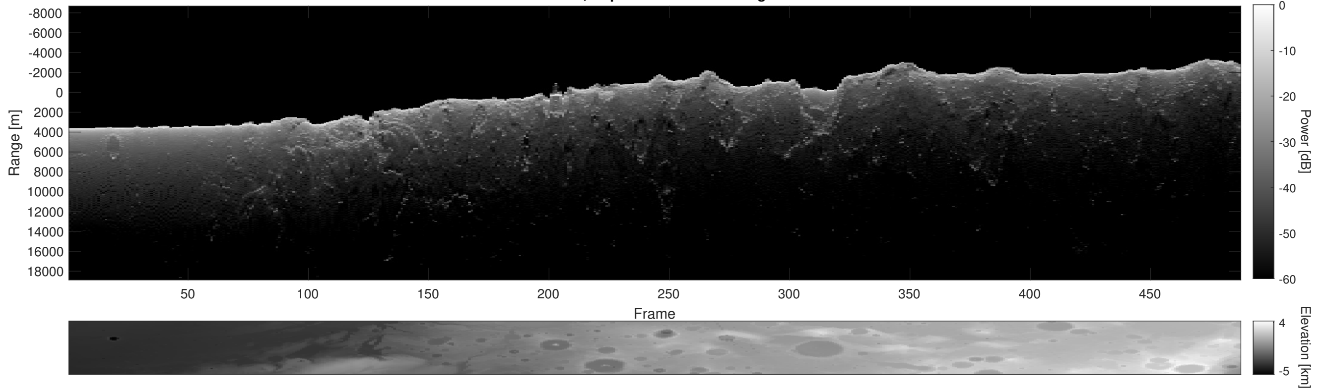
Orbit 6945, Depth-Corrected Cluttergram
