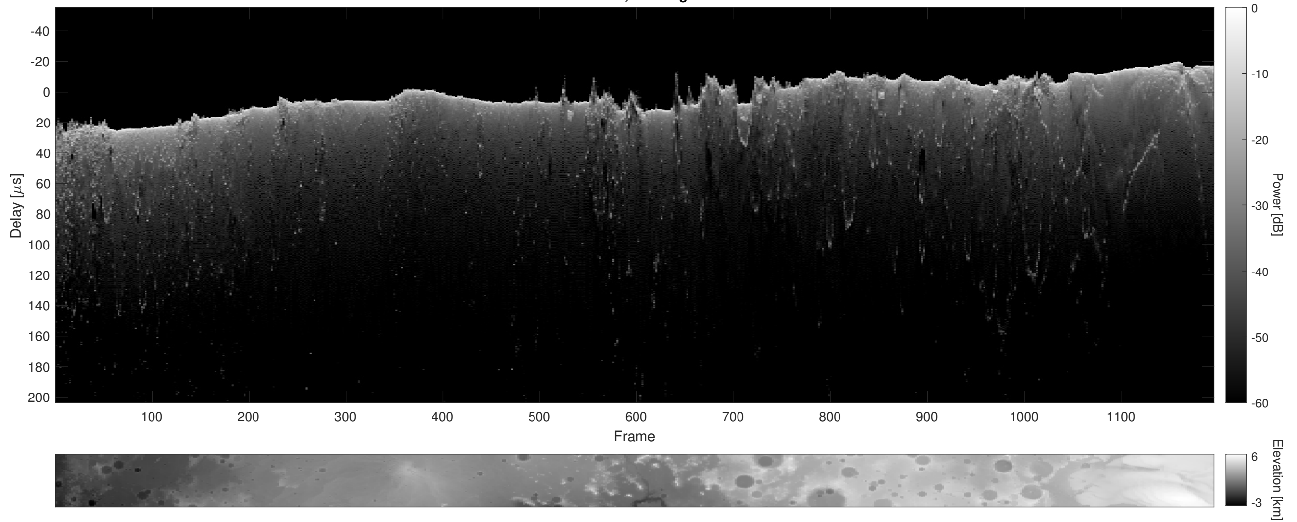
Orbit 6946, Cluttergram
