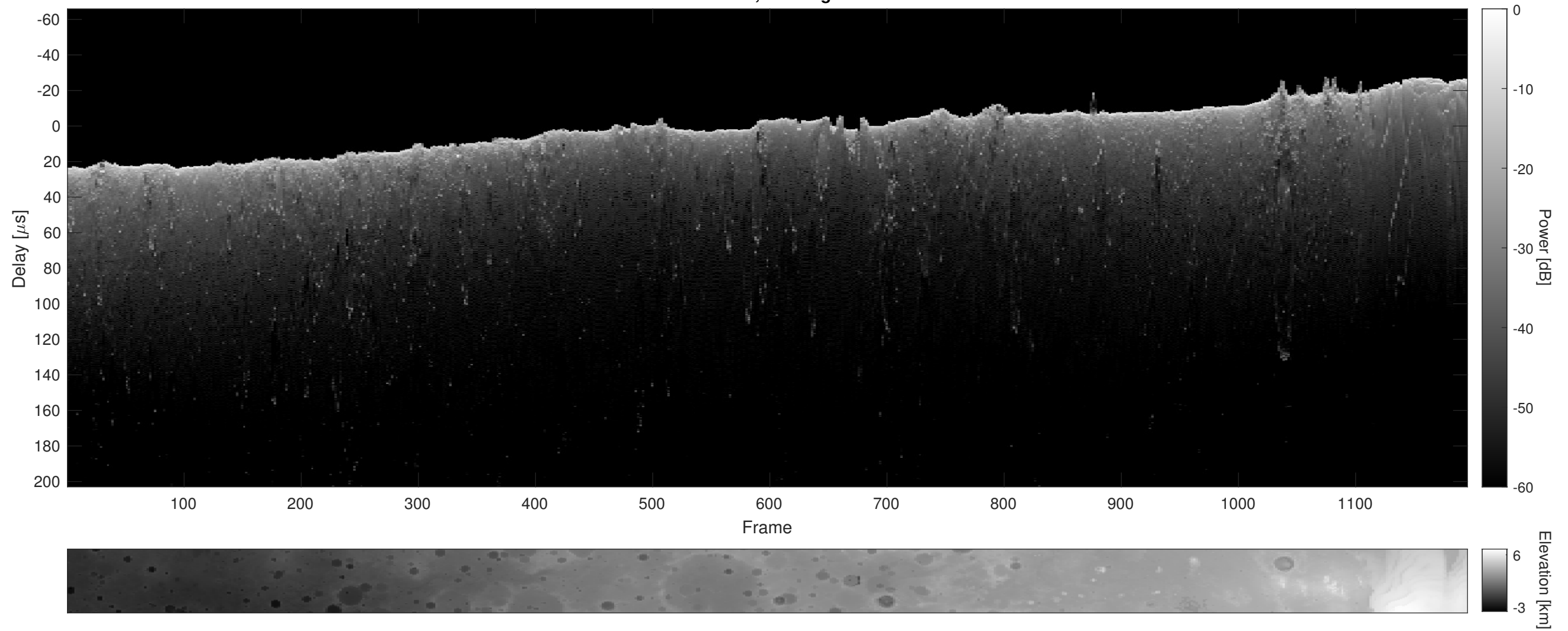
Orbit 6947, Cluttergram
