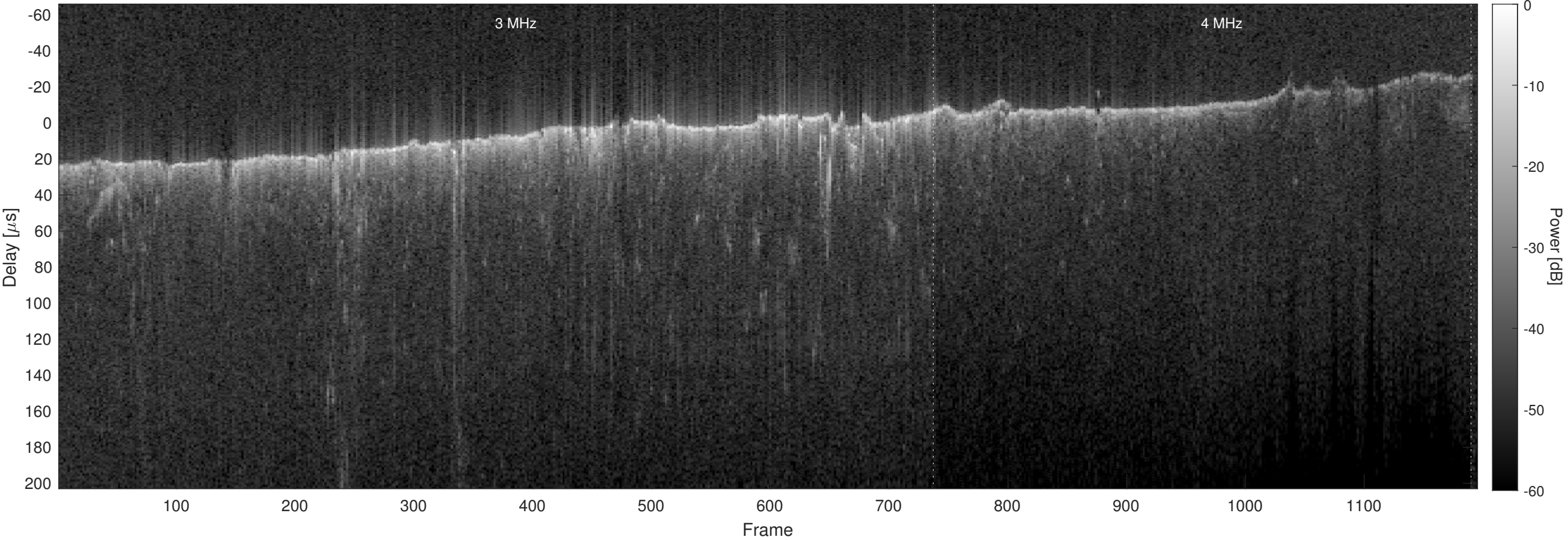
Orbit 6947, Optimized, No Window, Channel 2
