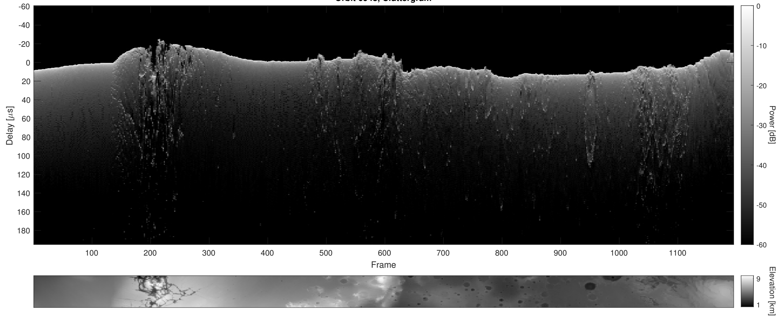
Orbit 6948, Cluttergram
