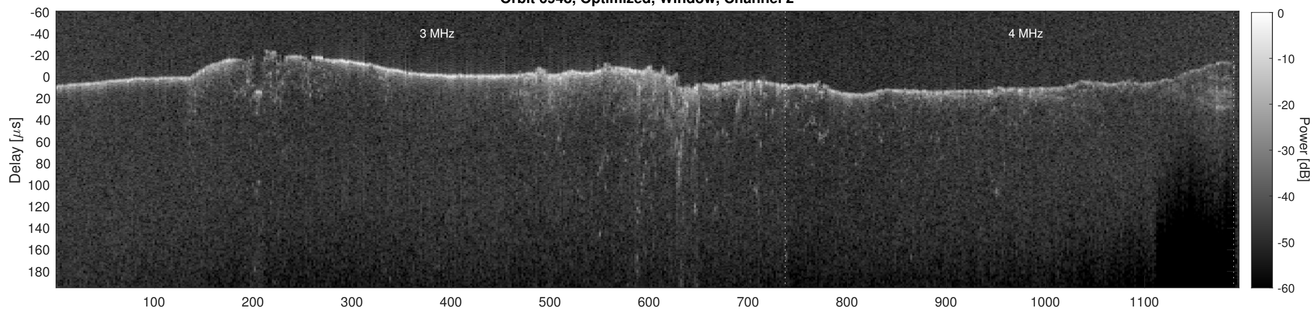
Orbit 6948, Cluttergram
