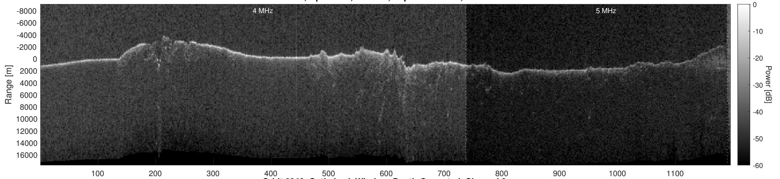
Orbit 6948, Optimized, Window, Depth-Corrected, Channel 2
