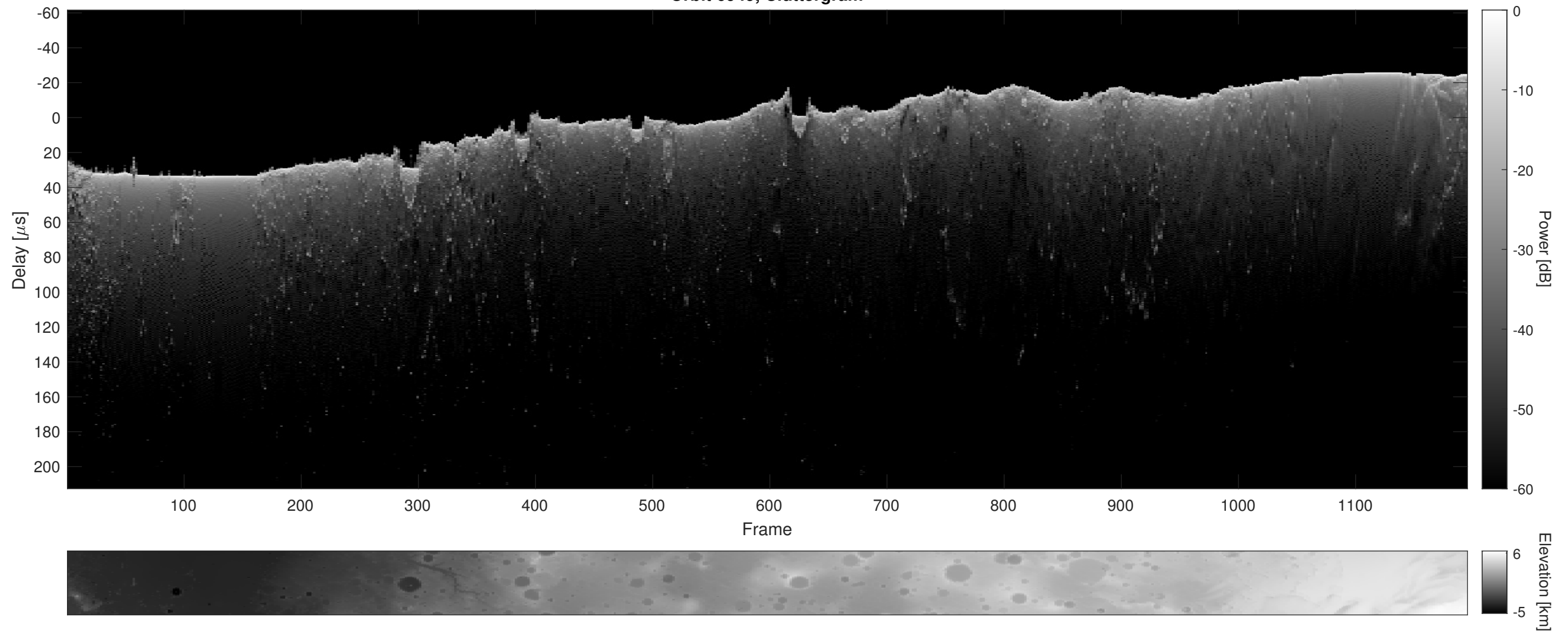
Orbit 6949, Cluttergram
