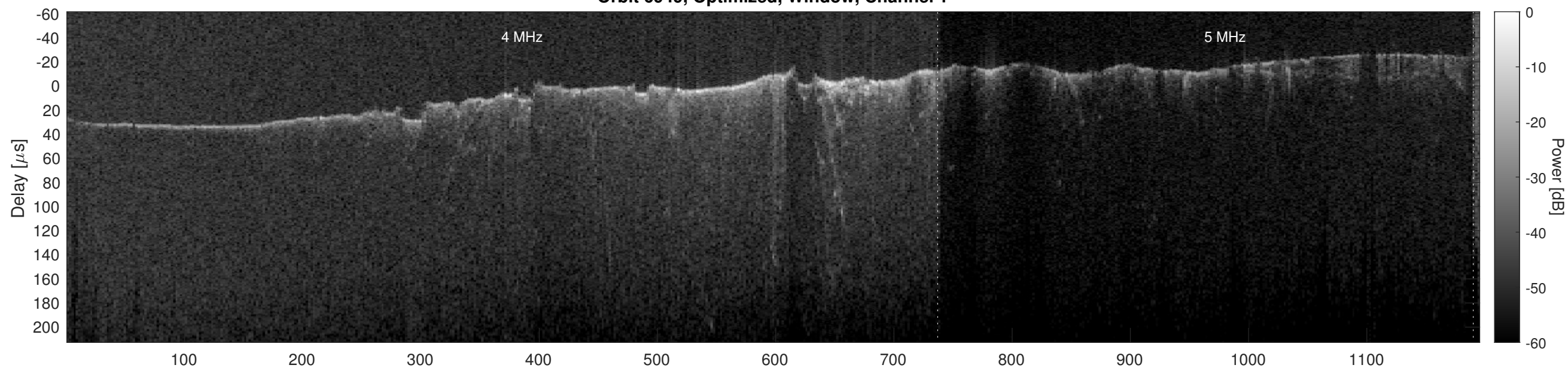
Orbit 6949, Optimized, Window, Channel 2
