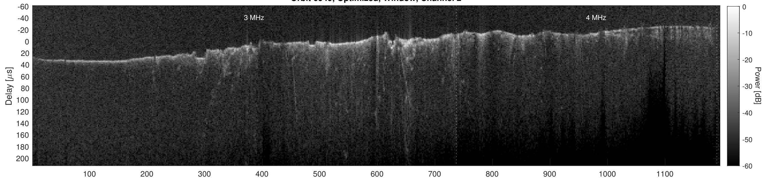
Orbit 6949, Cluttergram
