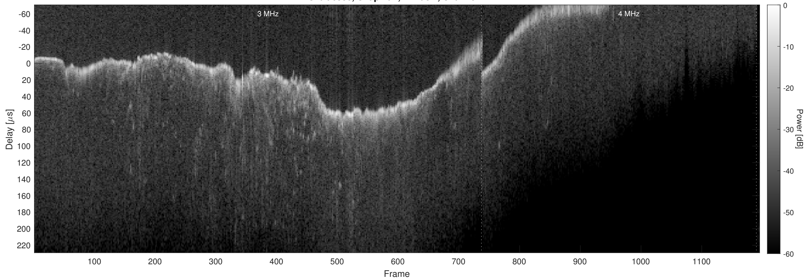
Orbit 6950, Chapman, Window, Channel 2
