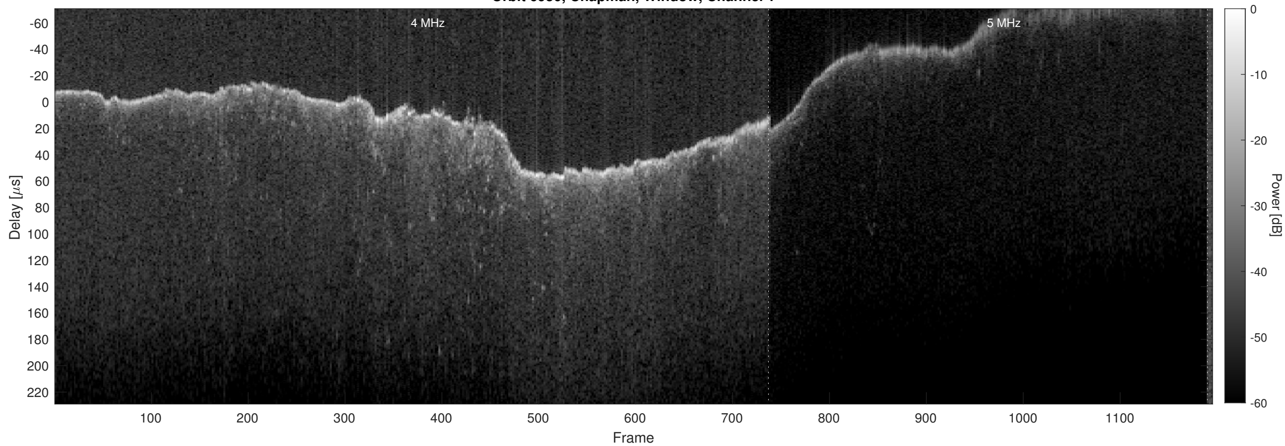
Orbit 6950, Chapman, Window, Channel 2
