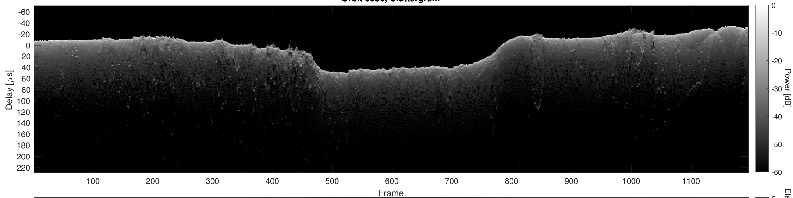
Orbit 6950, Cluttergram
