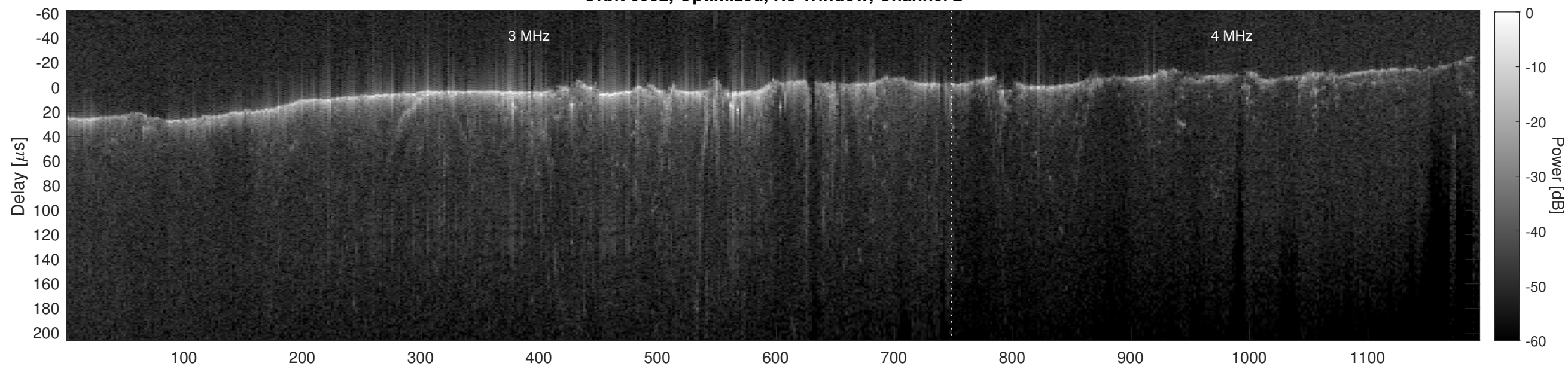
Orbit 6952, Cluttergram
