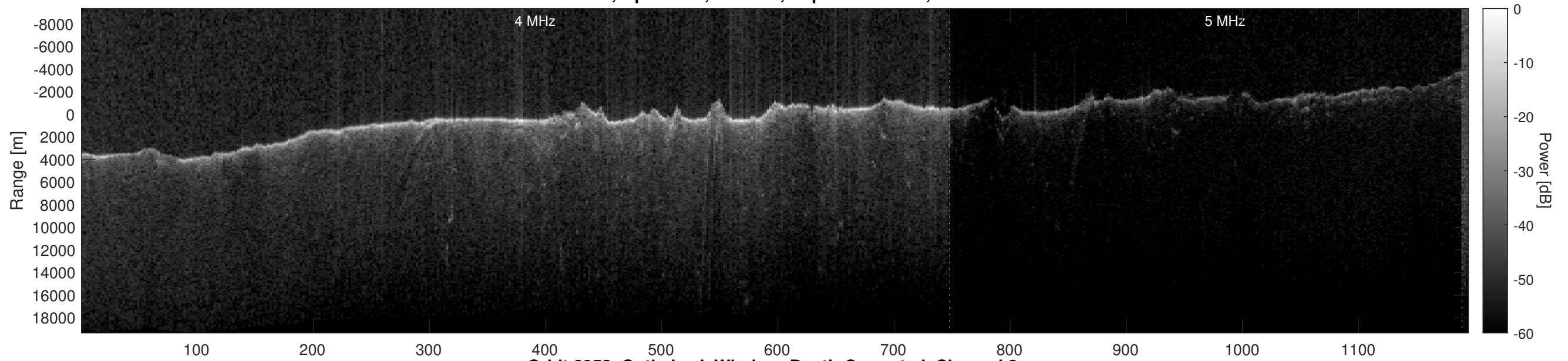
Orbit 6952, Optimized, Window, Depth-Corrected, Channel 2
