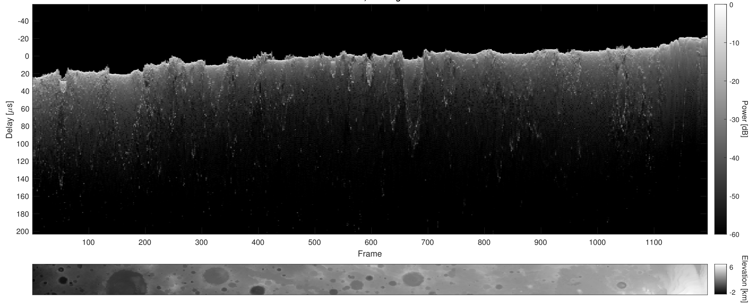
Orbit 6954, Cluttergram
