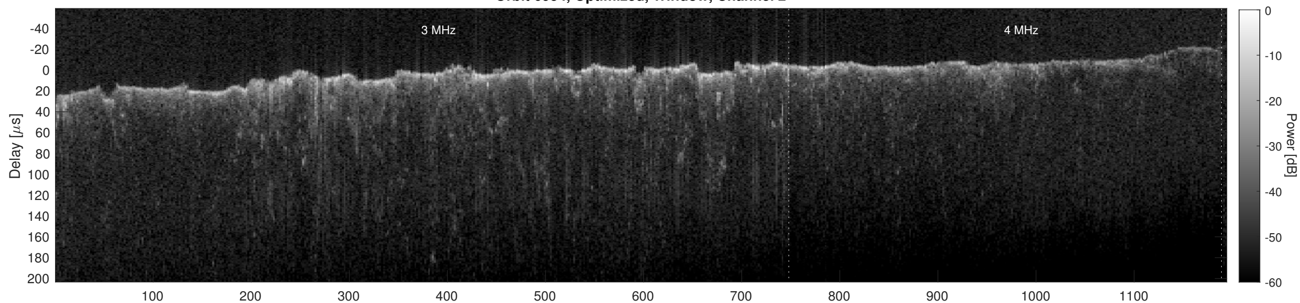
Orbit 6954, Cluttergram
