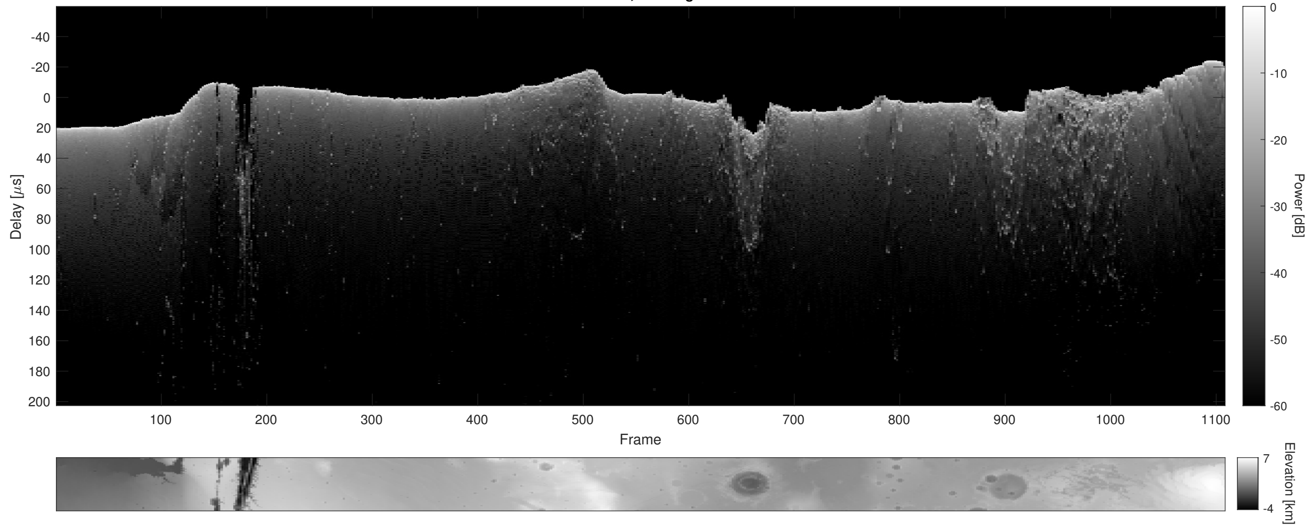
Orbit 6955, Cluttergram
