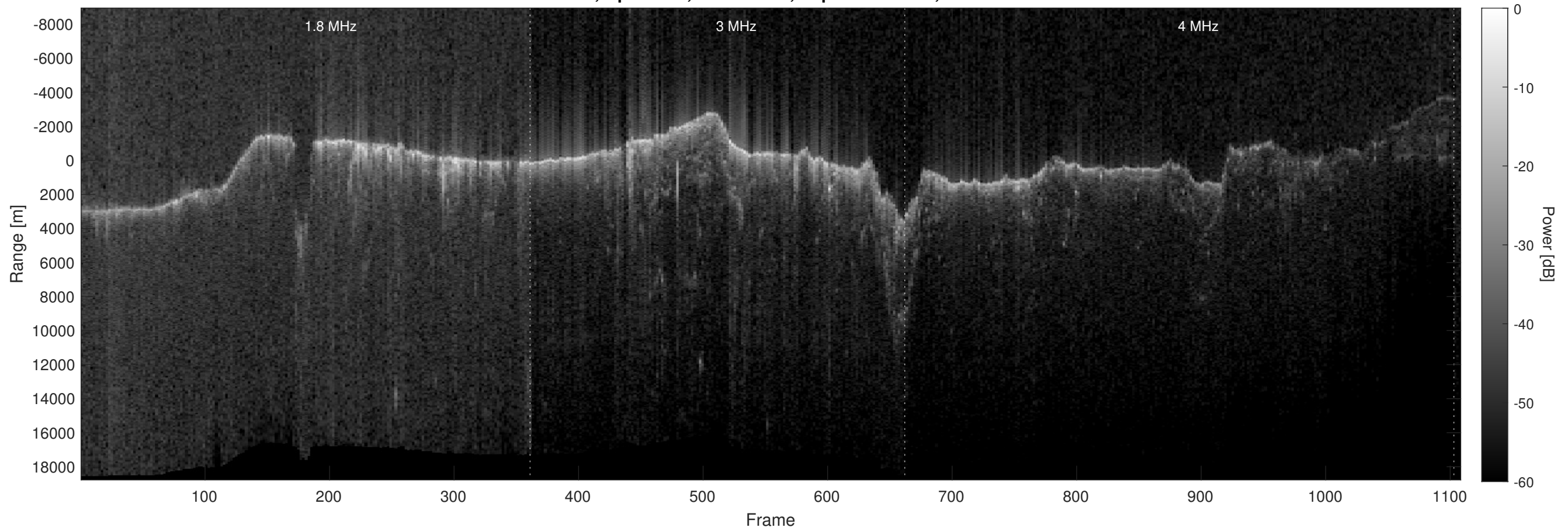
Orbit 6955, Optimized, No Window, Depth-Corrected, Channel 2
