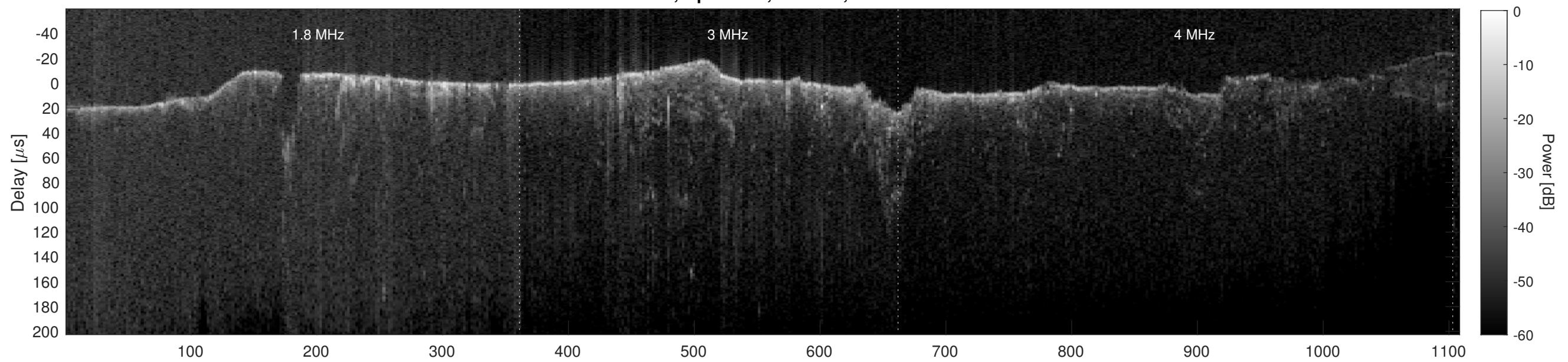
Orbit 6955, Cluttergram
