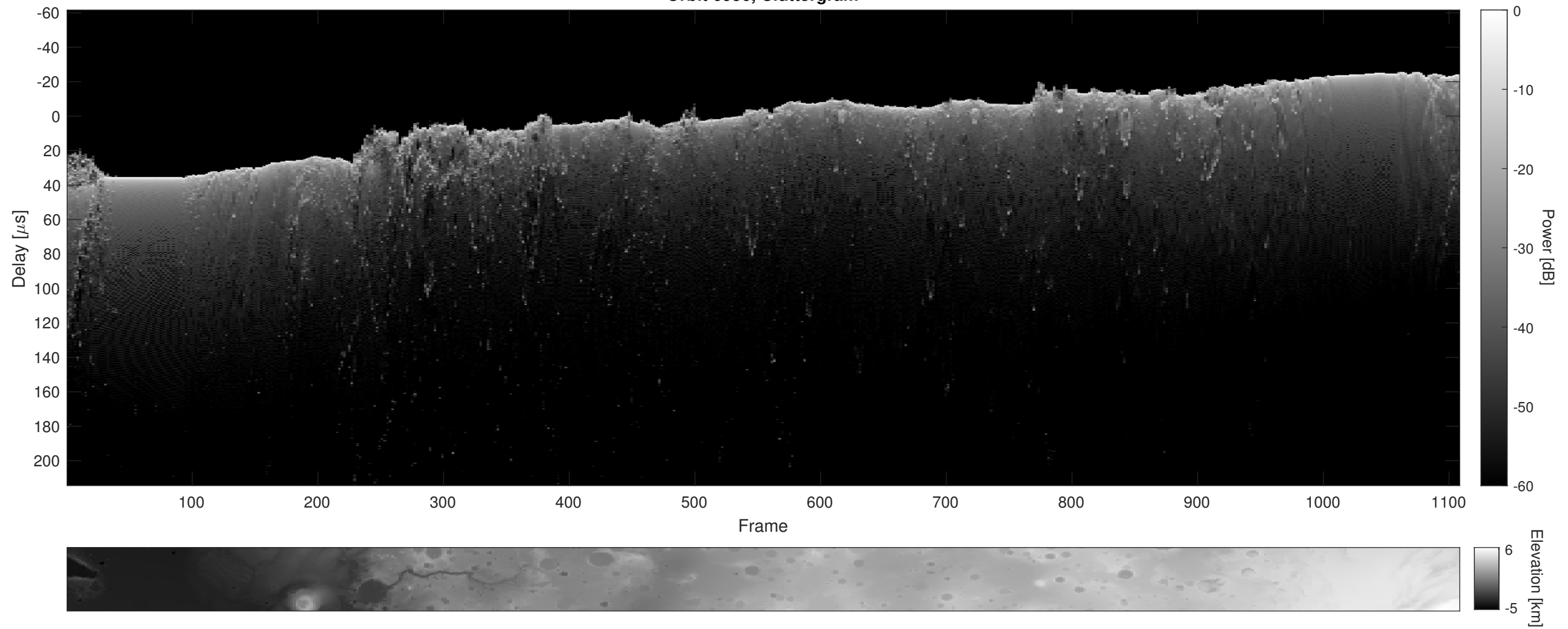
Orbit 6956, Cluttergram
