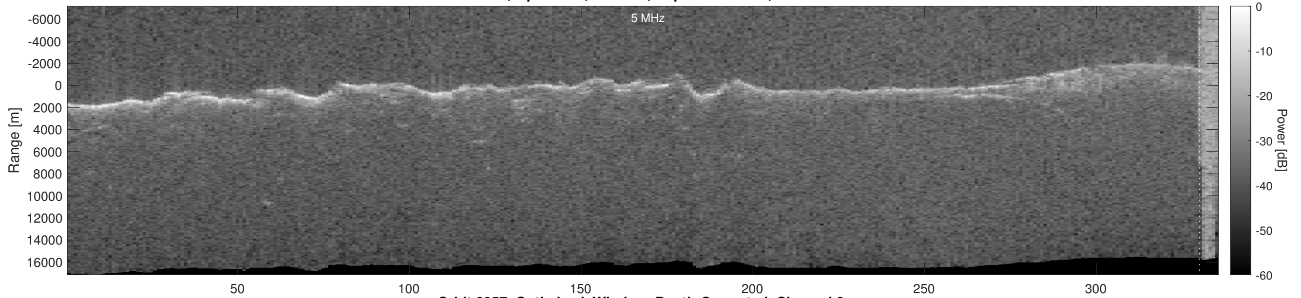
Orbit 6957, Optimized, Window, Depth-Corrected, Channel 2
