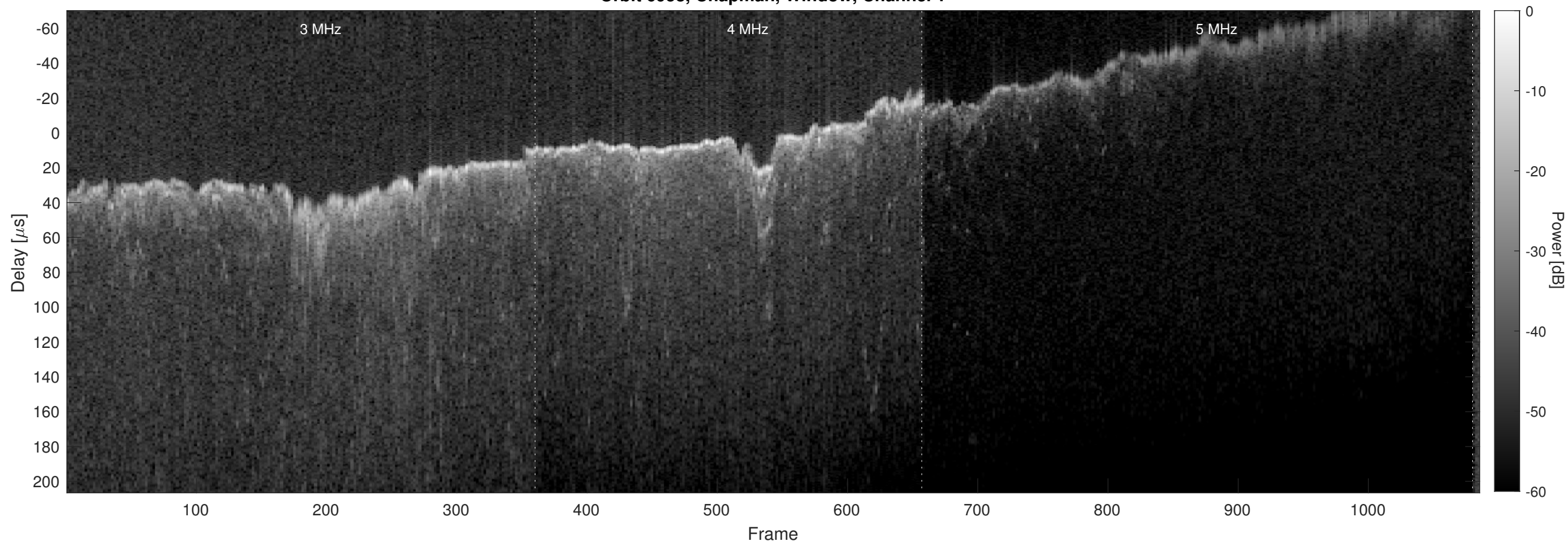
Orbit 6958, Chapman, Window, Channel 2
