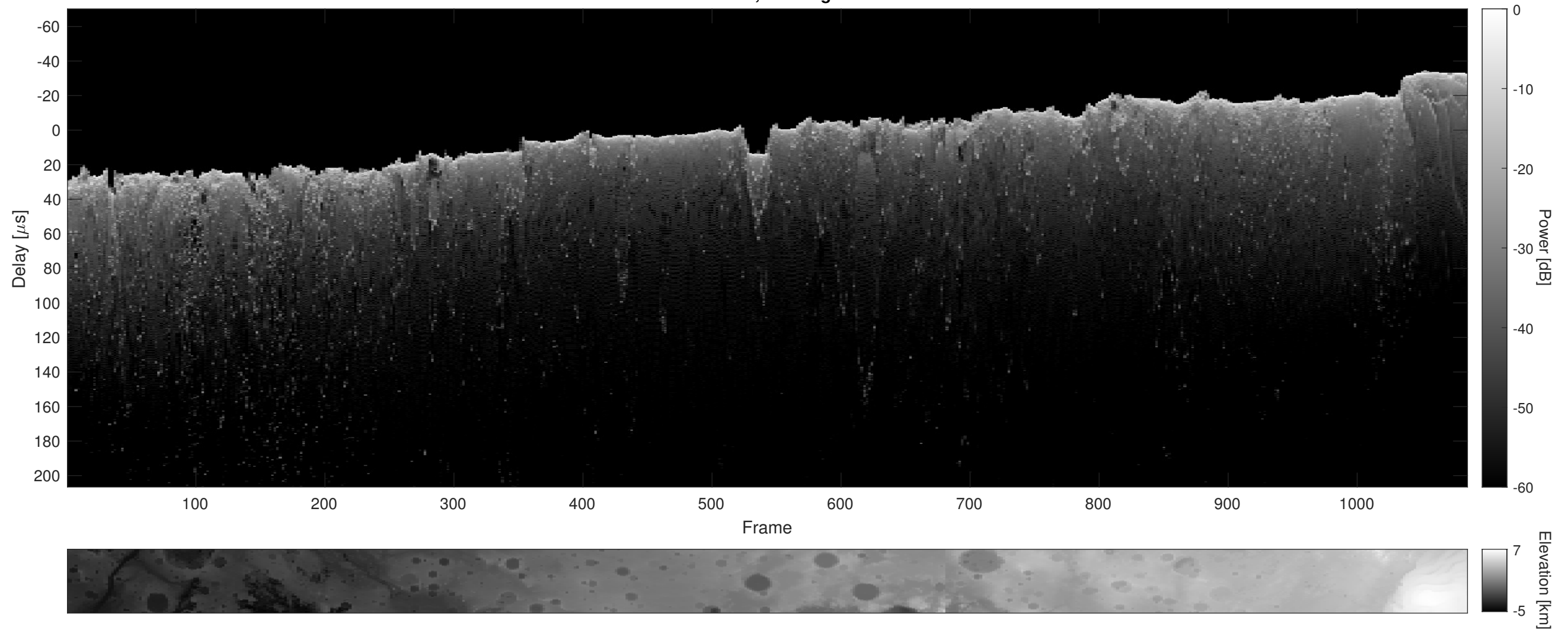
Orbit 6958, Cluttergram
