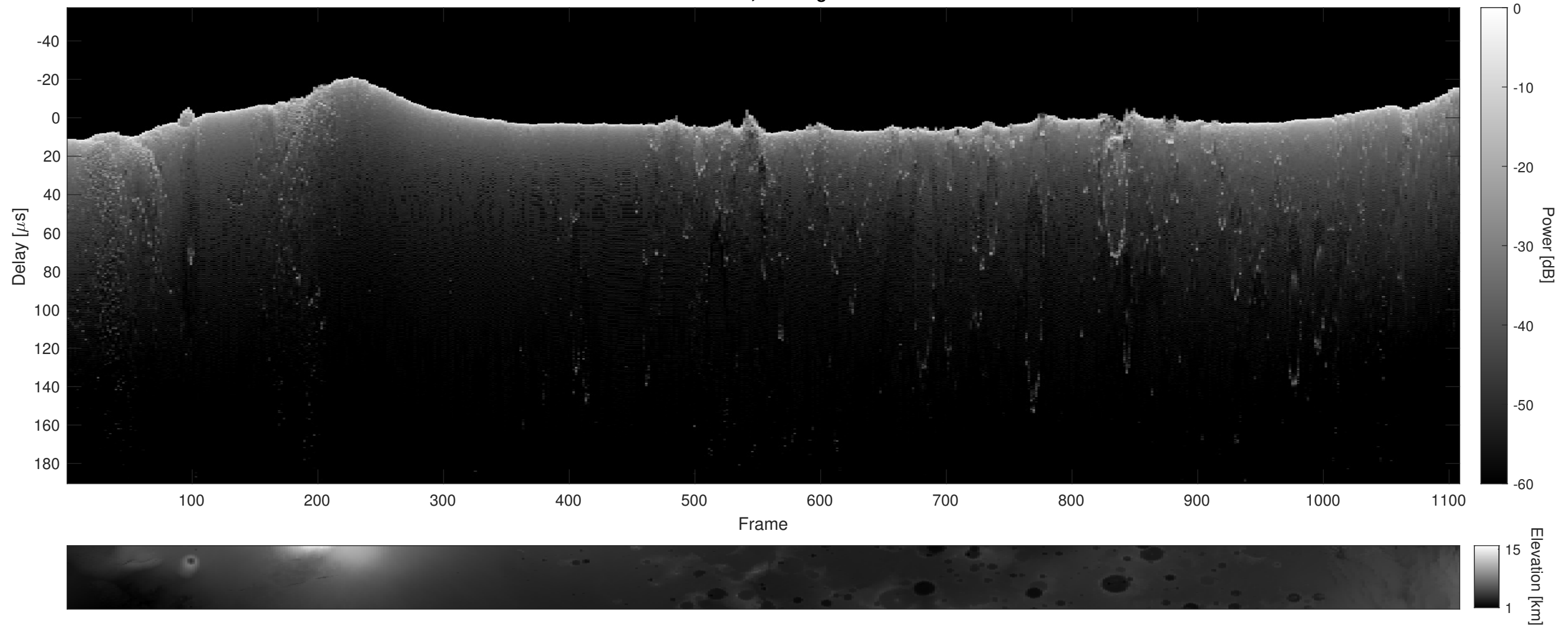
Orbit 6959, Cluttergram
