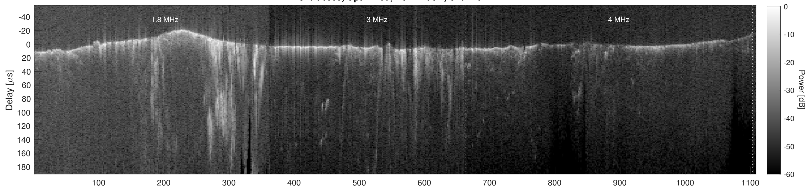
Orbit 6959, Cluttergram
