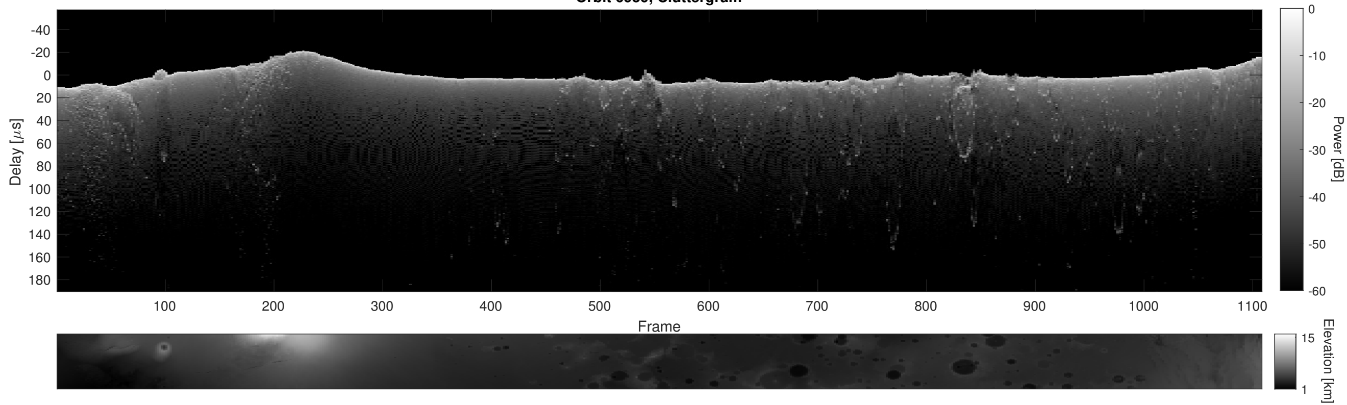
Orbit 6959, Cluttergram
