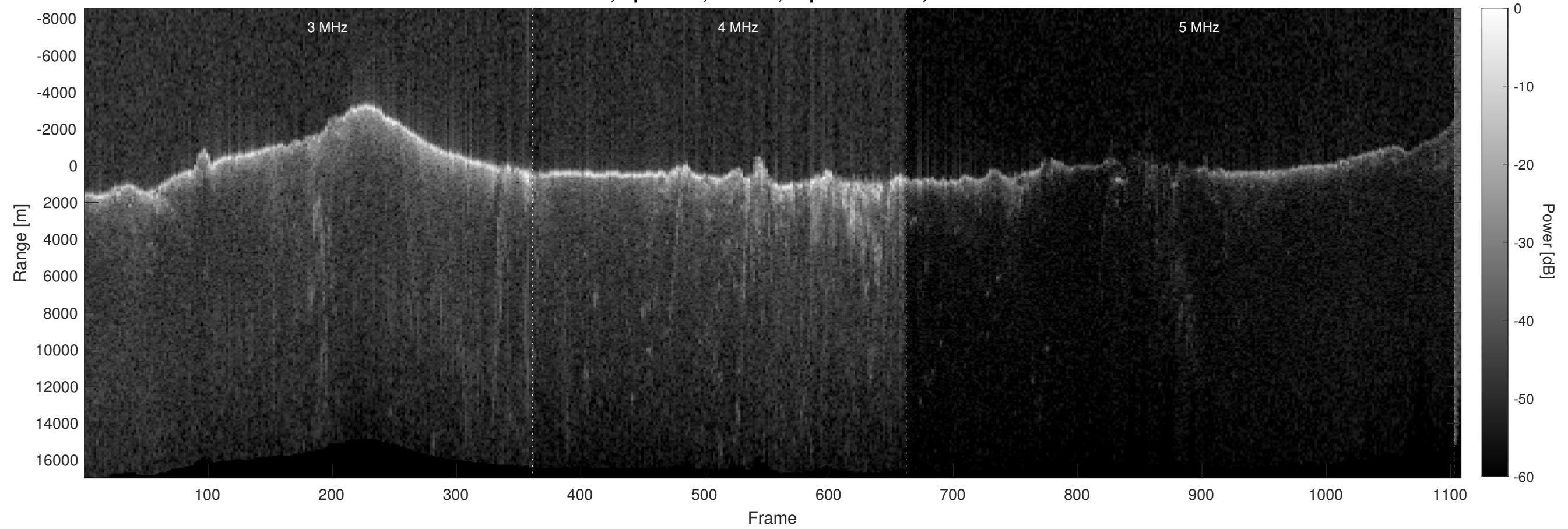
Orbit 6959, Optimized, Window, Depth-Corrected, Channel 2
