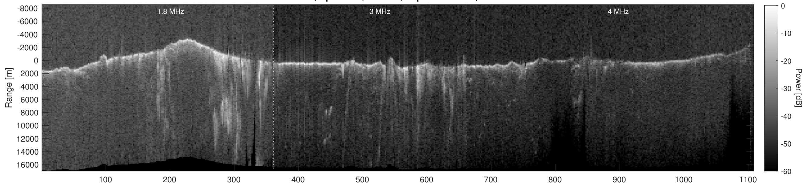
Orbit 6959, Depth-Corrected Cluttergram
