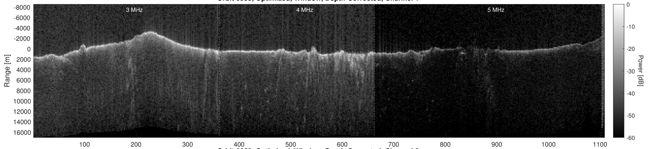
Orbit 6959, Optimized, Window, Depth-Corrected, Channel 2
